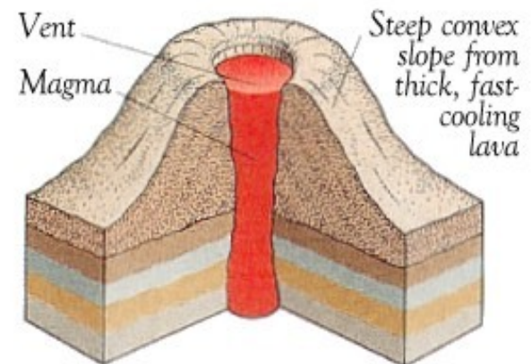
Dome volcano
