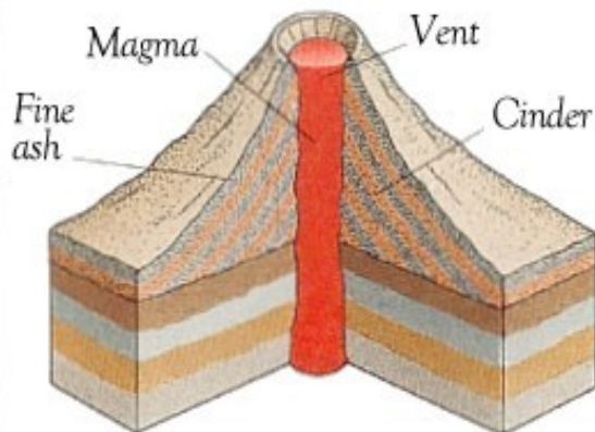
Ash-cinder volcano
