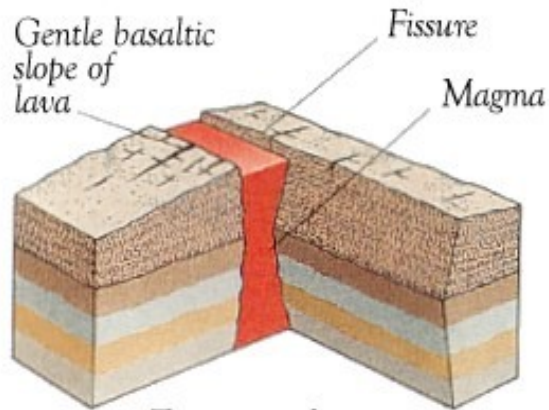
Fissure volcano
