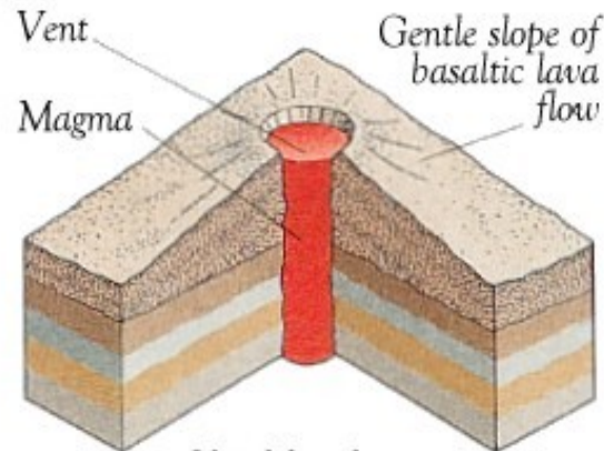
Shield volcano
