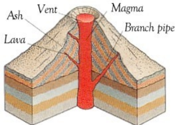
Composite volcano
